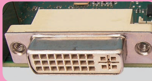
DVI-I Connector
